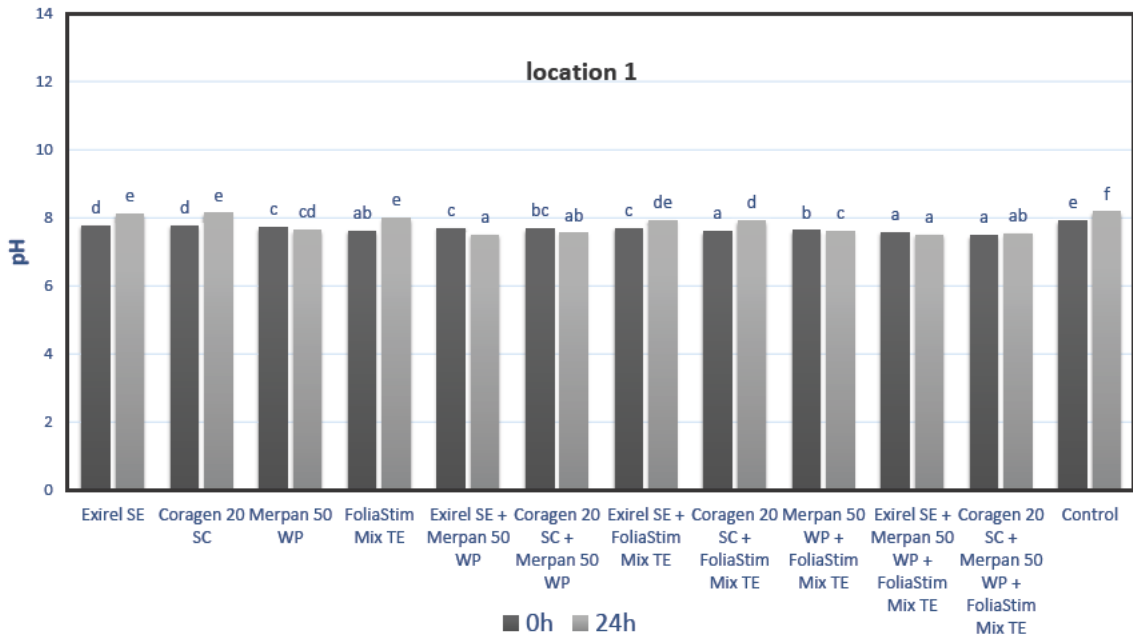
Figure 1. pH values of spray liquids of insecticides, fungicide, foliar fertilizer and their mixtures in well water immediately after mixing and after 24 h (location 1)
