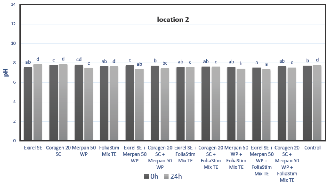
Figure 2. pH values of spray liquids of insecticides, fungicide, foliar fertilizer and their mixtures in well water immediately after mixing and after 24 h (location 2)
