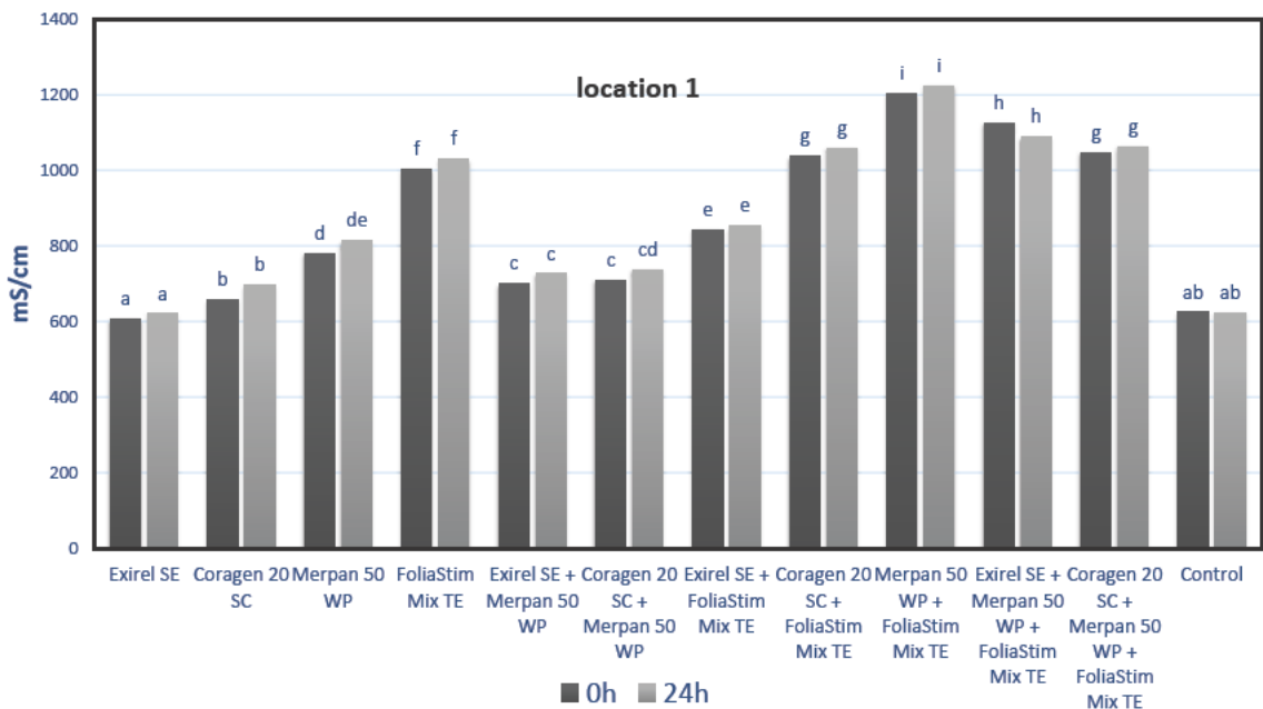
Figure 5. Electroconductivity of insecticides, fungicide, foliar fertilizer and their mixtures in well water immediately after preparation and after 24 h (location 1)
