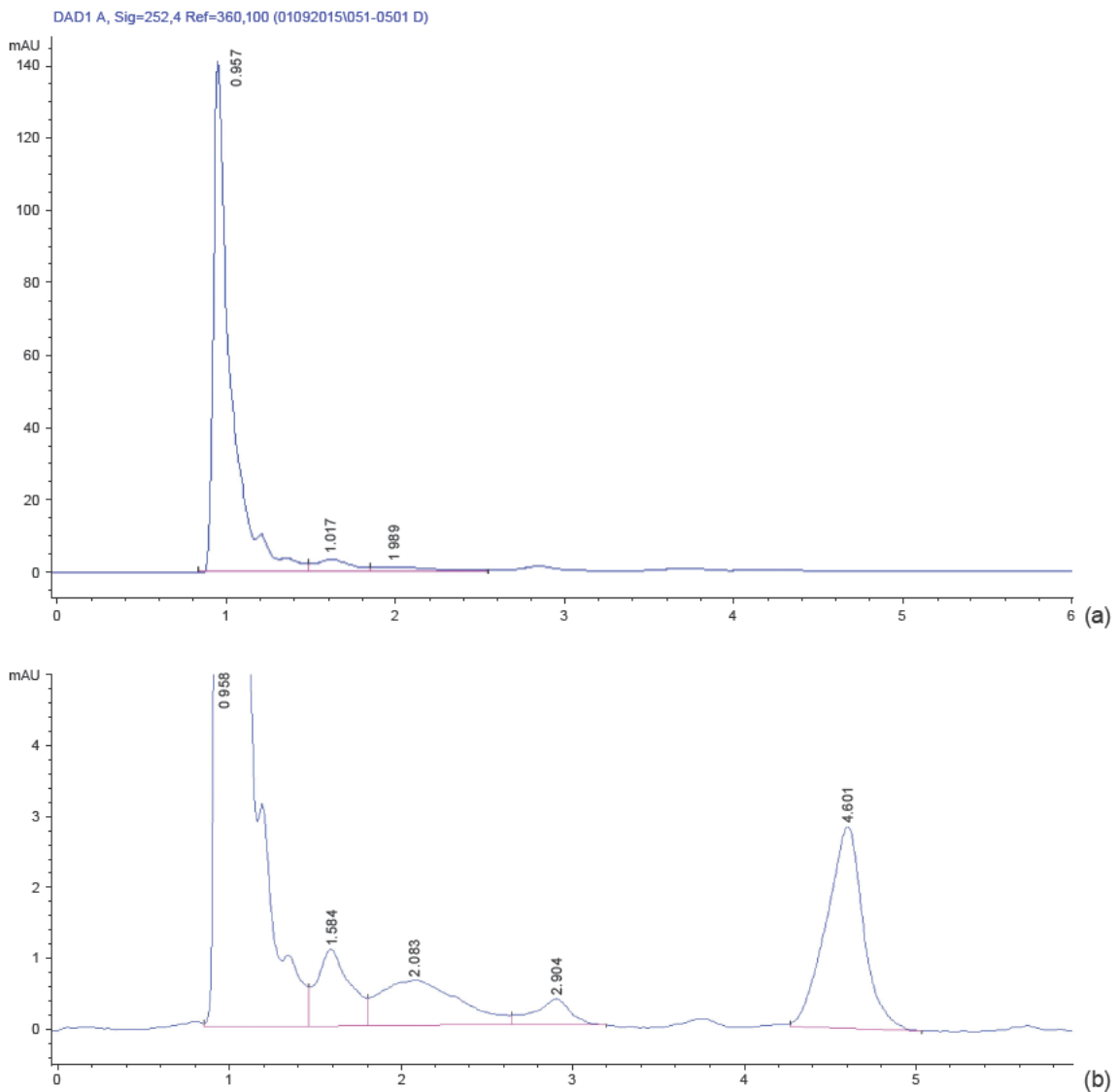
Figure 3. Chromatogram of the control sample (a) and matrix fortified with thiacloprid (b)
